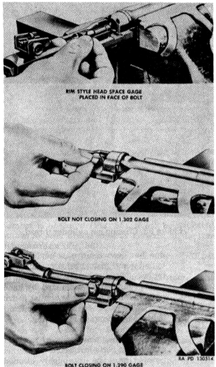
Figure 82. Checking head space.
