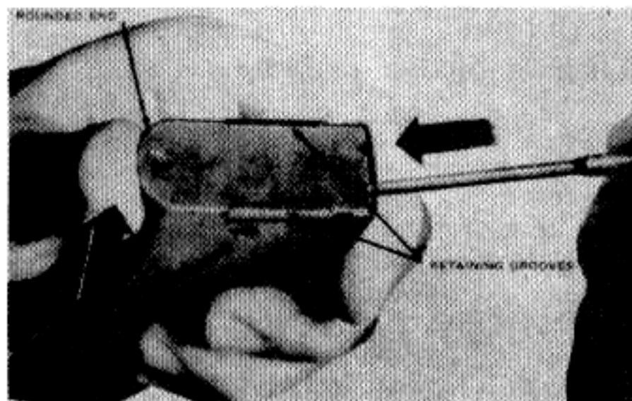
Figure 33. Removing the magazine base.
