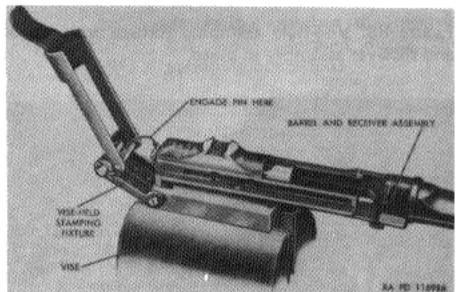
Figure 87. Placement of barrel and receiver assembly in vice-held stamping fixture.
