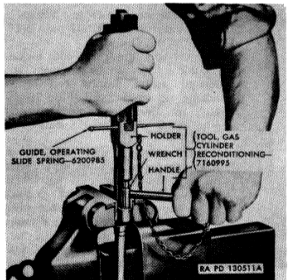
Figure 77. Removing piston nut from gas cylinder.
