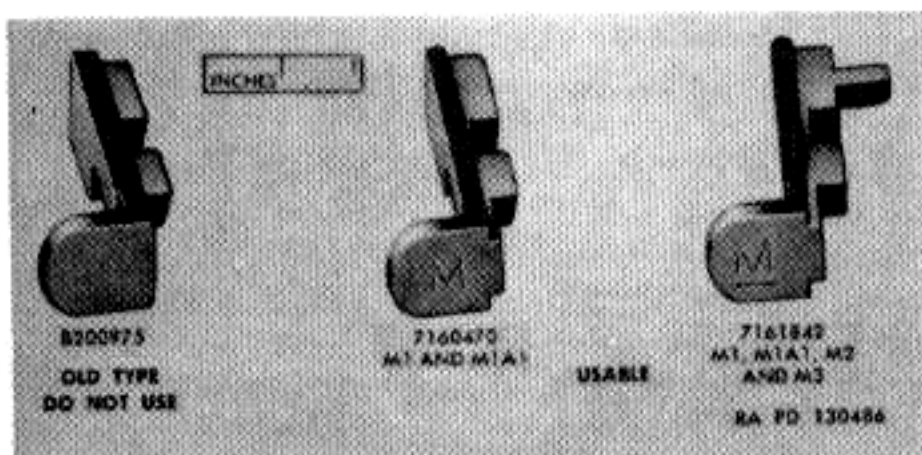
Figure 54. Magazine catches.
