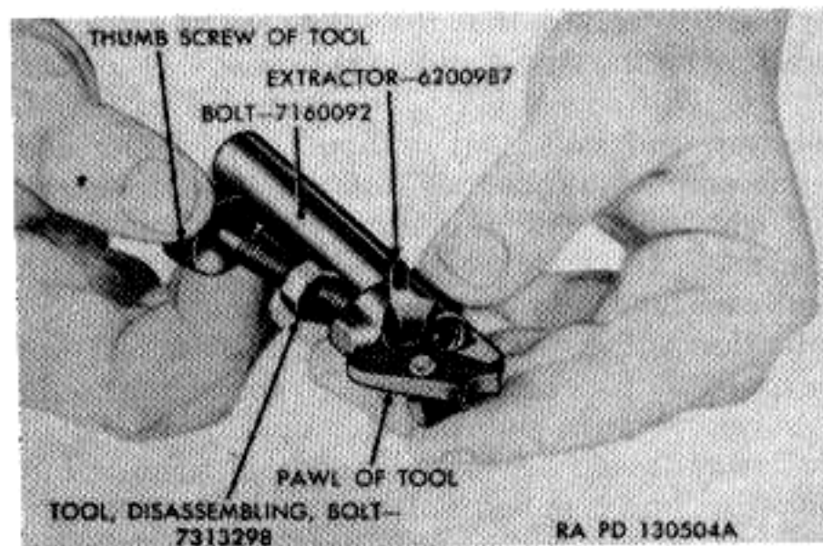
Figure 60. Disassembling bolt.
