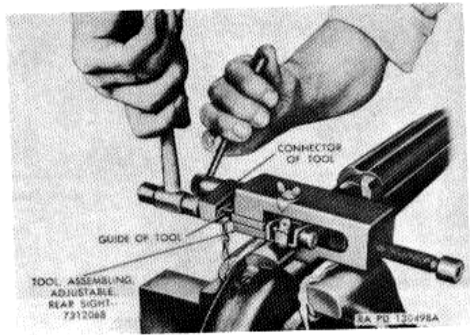
Figure 68. Removing adjustable rear sight.
