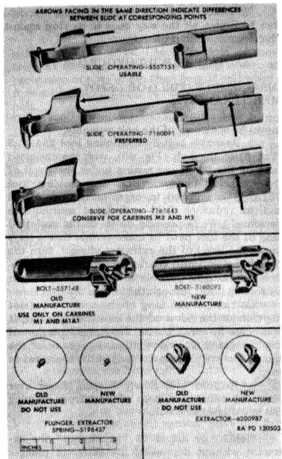
Figure 58. Slide, bolt, extractor and plunger.
