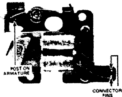
Figure 22 Combination-magnet assembly
