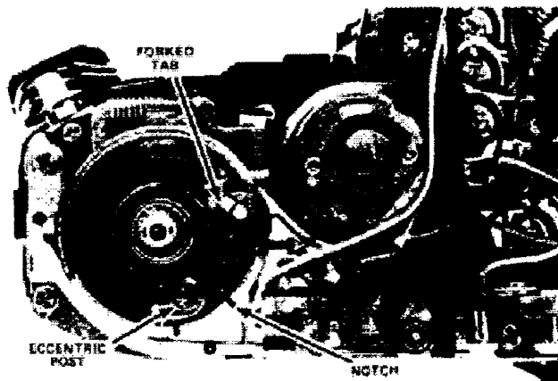
Figure 38 Speed knob removed
