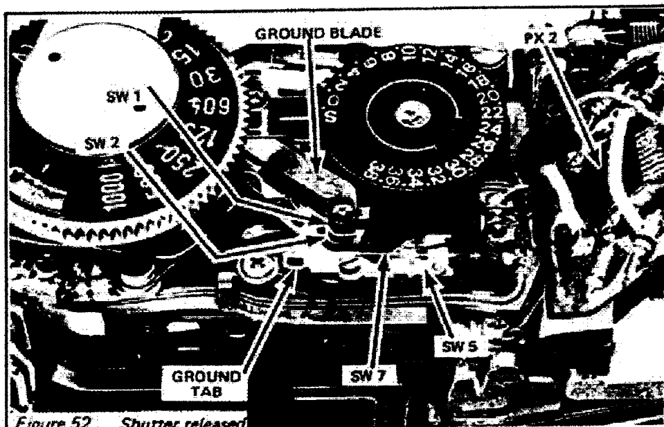
Figure 52 Shutter released
