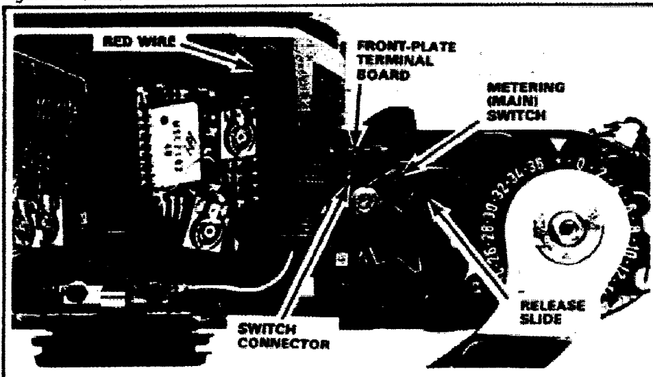
Figure 4 Pentax ME
