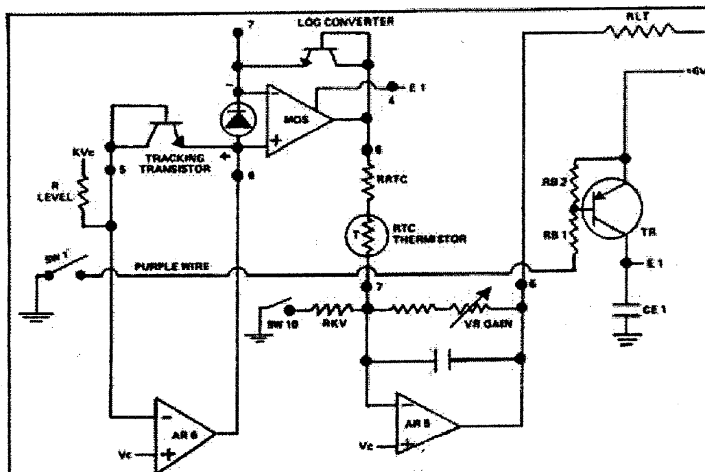
Light-measuring circuit
